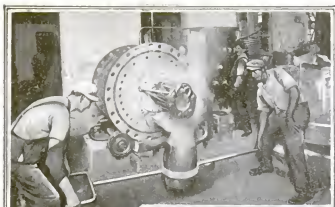
The molten brass is being poured from the electric furnace; the man at the switchboard controls the flow
