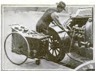
The electrical test-cart is the first thing of its kind in the way of a complete apparatus for testing any part of the electrical mechanism of automobiles, trucks, and tractors
