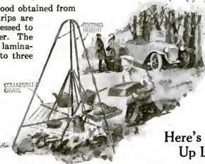
Here is a collapsible stove for campers. The grate is mounted on a rod and opens up umbrella fashion
