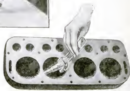
The method of using a recently invented gage for measuring the inside diameter of automobile engine cylinders is shown above
