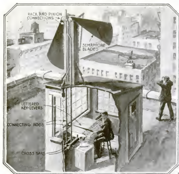
The operator of this mechanical semaphore spells out his messages by pressing down levers representing the letters of the alphabet
