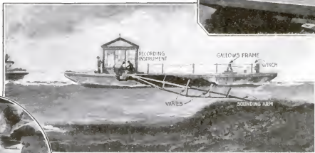
Above is shown the barge, equipped with sounding and recording mechanism used by government engineers in making profile maps of the river bed along the upper Mississippi. The operation of the machine is shown at left. Note the vanes that steady the lower end of sounding arm on the river bottom.
