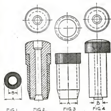
Why buy a punch to cut out washers when you can easily make the one illustrated which serves a double purpose?
