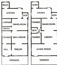
ORIGINAL PLAN Remove the old pantry partitions and build in a bath-room opening conveniently into the two bedrooms
