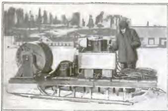
This is an electrical machine used for thawing the ground in Alaska, where a railroad was to be built
