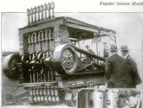
In crushing a cement road, a battery of heavy plungers, with removable chisel-shaped points, shown at right, are raised and lowered by eccentric levers on a shaft driven by the truck motor
