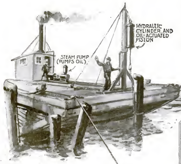
Piles may be pulled out of deep water, by mounting pump and spar on a scow. The device has a lifting power of eight tons
