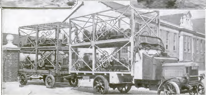
How a British automobile manufacturer delivers eight auto chassis to the body builders in one haul. Four of the chassis are carried on a two-story steel framework structure on the truck, the remaining four on a trailer
