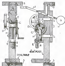
The whole machine is bolted to a strong post so that it will carry the motion block to its highest point
