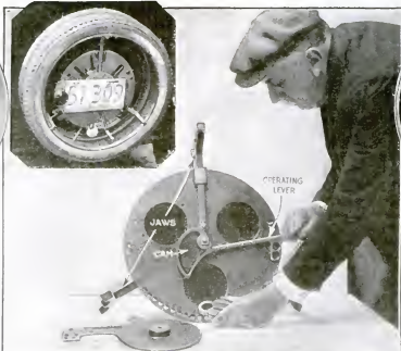
A new thief-proof tire holder consists of a disk with three radial sliding arms that push outward to engage the rims of the tires by a centrally pivoted lever with an eccentric cam. A series of holes along the rim of the disk make it possible to padlock the handle of the lever when the jaws have a firm hold on the tires
