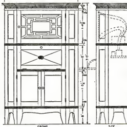
A walnut radio cabinet with inlays. Additional working details and a complete bill of materials are contained in Home Workshop Blueprint No. 16.
