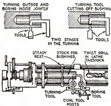
With this double tool set-up the bushings are turned and bored at the same time
