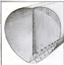
Cross section of the semi-rigid "R-1," showing double envelope that will inclose helium filled balloons, and rigid, three-cornered framework keel of duralumin that will run the entire length of the ship
