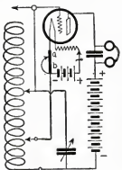
FIG. 2 Wiring diagram used in hooking up the parts
