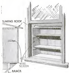
The side view and front of the box show how easily it can be constructed. It will save you a big ice bill, too
