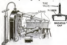
How air pressure makes leaks visible
